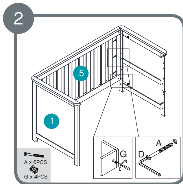
Assemble side using 6 x A bolts Assemble locking nuts 4 x G.
